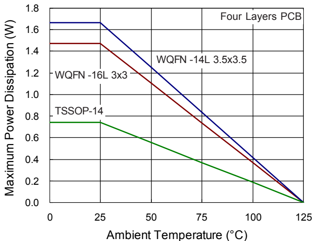
Figure 5. Derating Curves for RT8209A/B/C Packages
