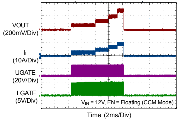
Power On in Short Circuit
