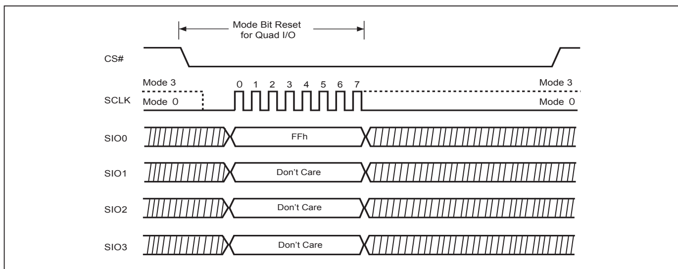
Figure 36. Performance Enhance Mode Reset for Fast Read Quad I/O (SPI Mode)
