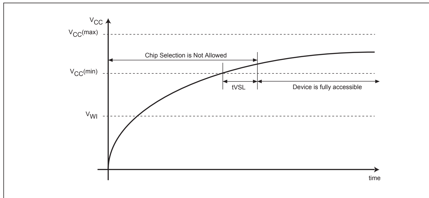
Figure 83. Power-up Timing
